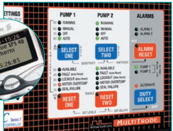
Detail of alarm on the pump controller
